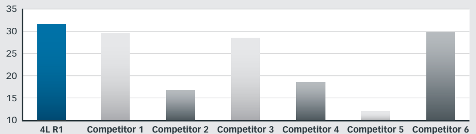
Original Tread Depth (OTD) @ center in mm for 405/70-20
